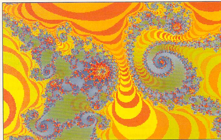
Figure 4. Tight Mandelbrot zoom with banded coloration.
