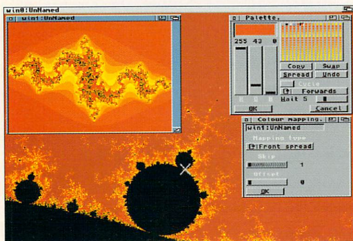
Figure 7. "X" marks the spot on the Mandelbrot set that generates this colorful Julia set. Also shown is Mand2000's color-palette control window.
