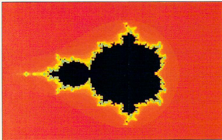
Figure 3. A MathVISION view of the entire Mandelbrot set.
