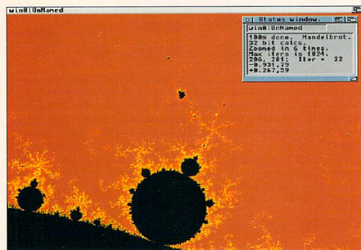
Figure 9. Mand2000 generates the classic Mandelbrot image from the cover of the August 1985 issue of Scientific American that launched "Mandelbrot Mania."
