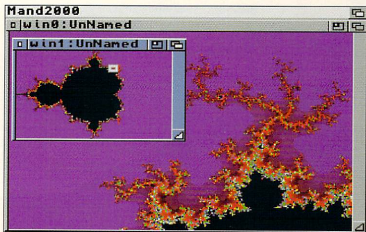
Figure 5. Mand2000 shows the location of a zoom window.
